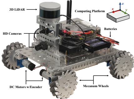
HydraOne Platform: E2M
