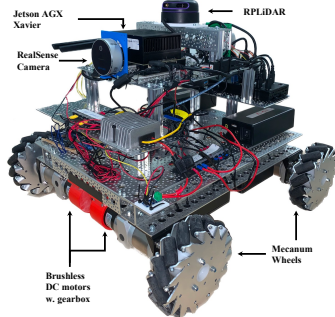
Donkey Platform: energy-efficient path planning, pNav
